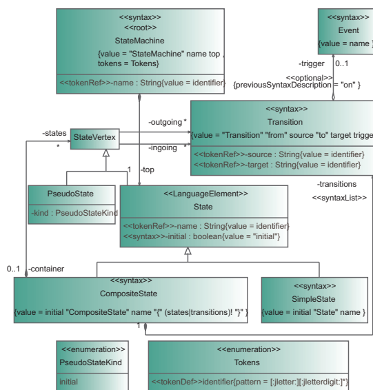
Figure 5: An annotated abstract syntax model for the State-Chart language.
