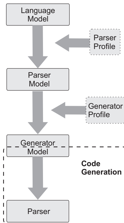
Figure 7: Parser development for a target language with the MetaCET's approach.
