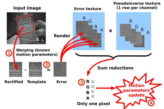
Figure 1: Tracking algorithm.
